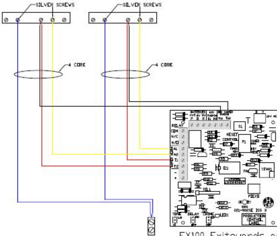
EX100 Exitguards and DoorWatcher
